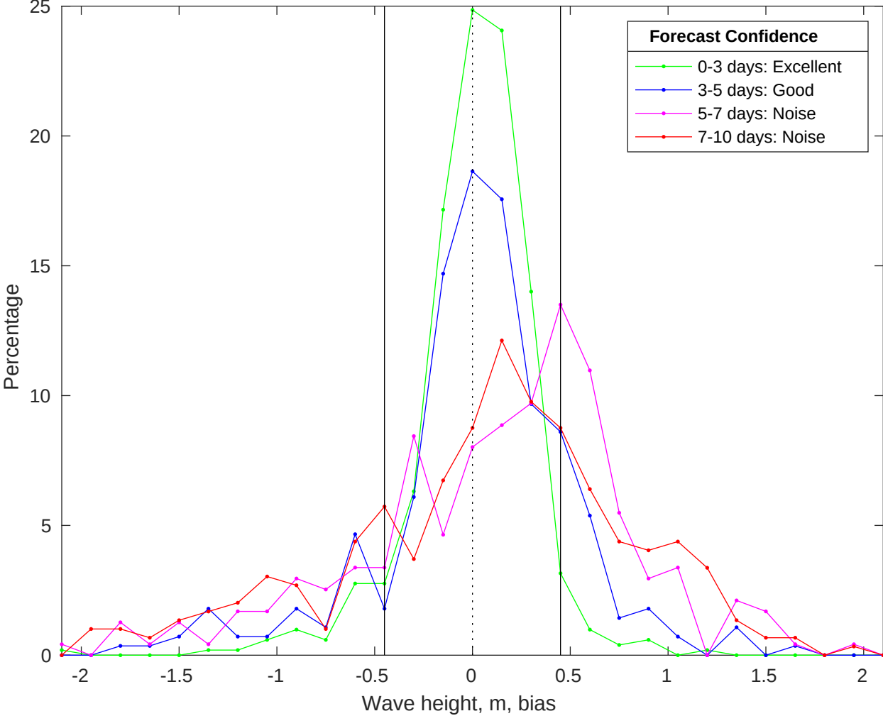
NDBC 46059 vs CMEMS Waves Bias Histogram: 10-Jan-2026
