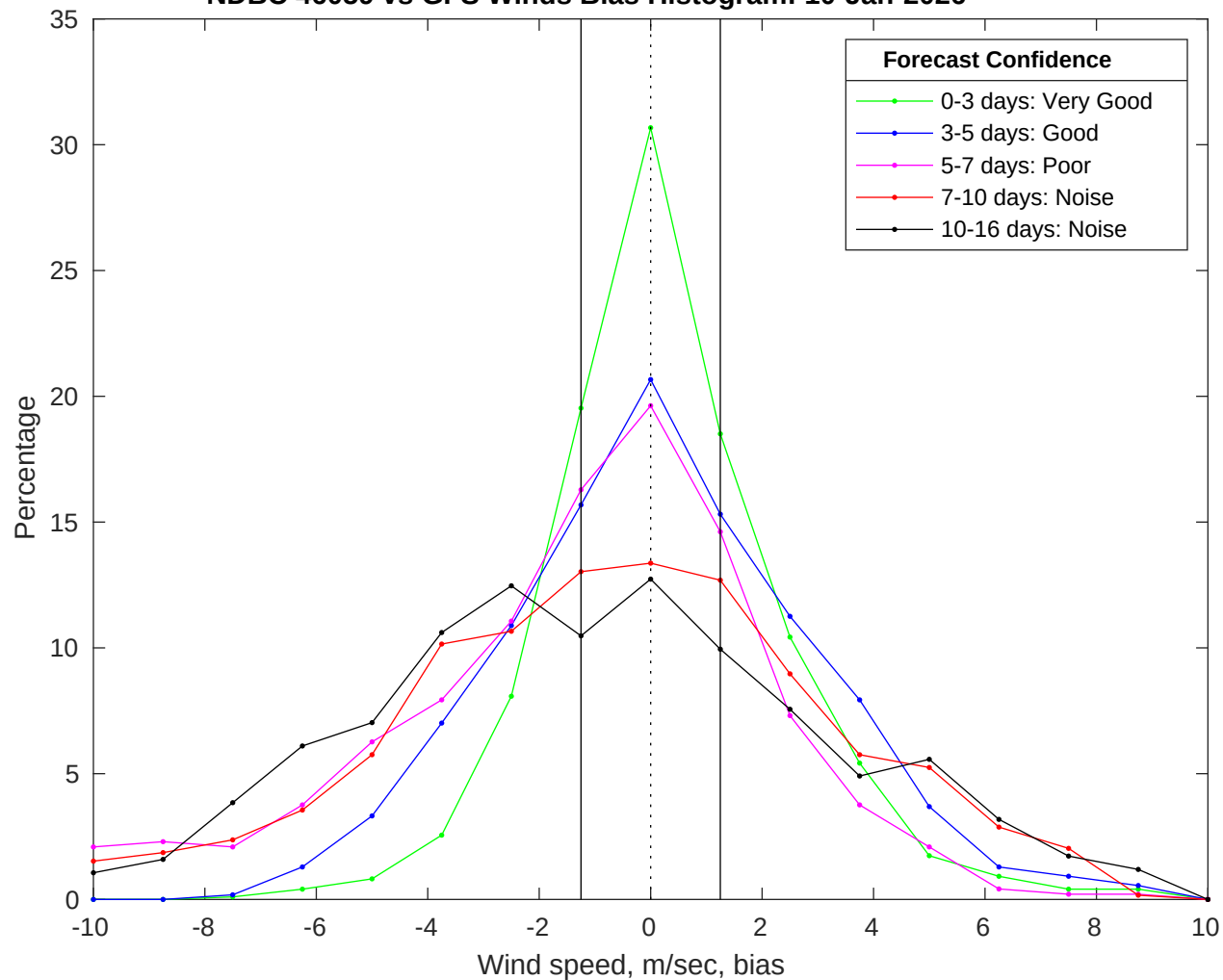
NDBC 46059 vs GFS Winds Bias Histogram: 10-Jan-2026
