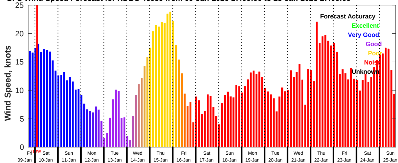
GFS Wind Speed Forecast for NDBC 46059 from 09-Jan-2026 17:00:00 to 25-Jan-2026 17:00:00
