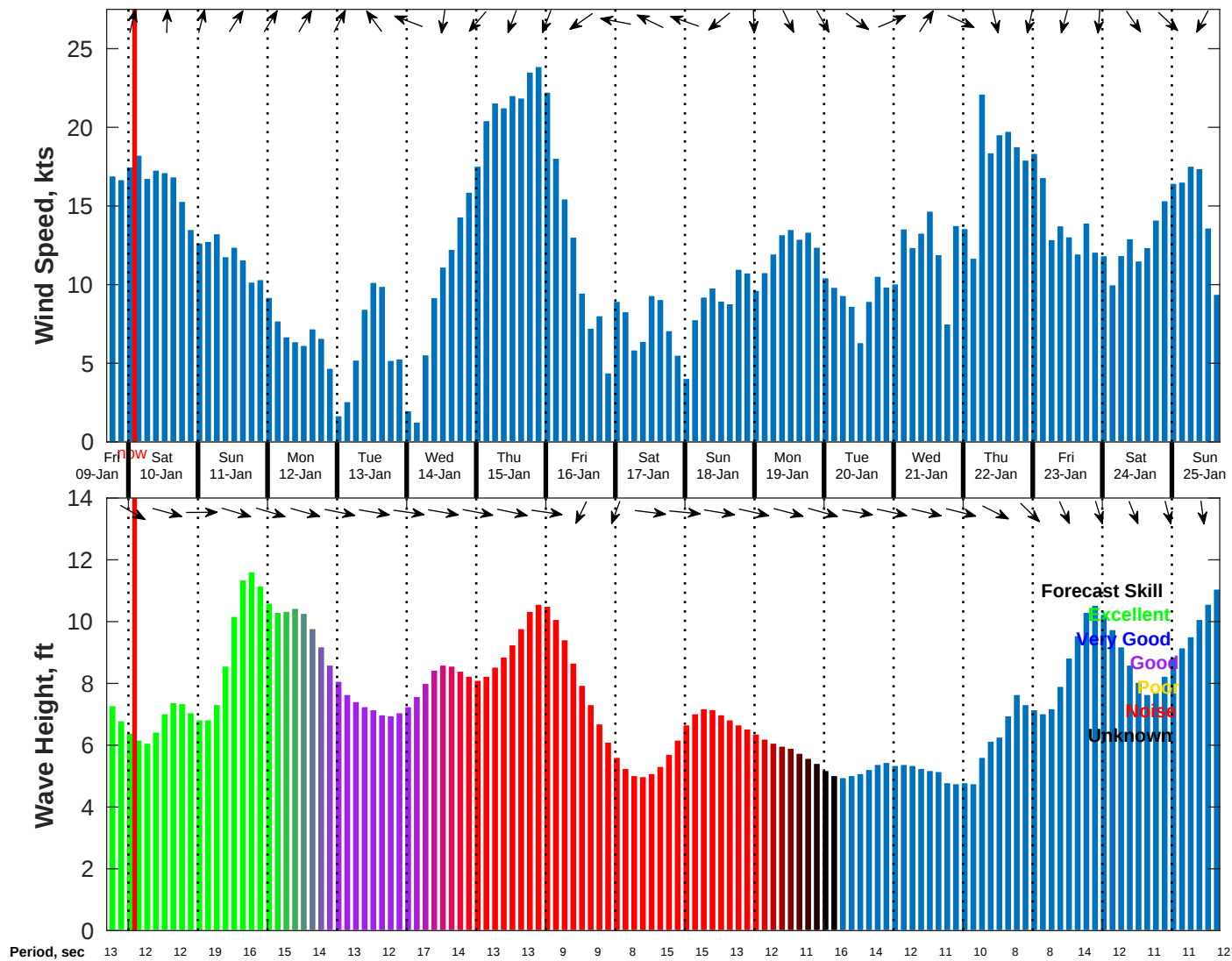
Wind & Wave Forecast for NDBC 46059 from 09-Jan-2026 17:00:00 to 25-Jan-2026 17:00:00
