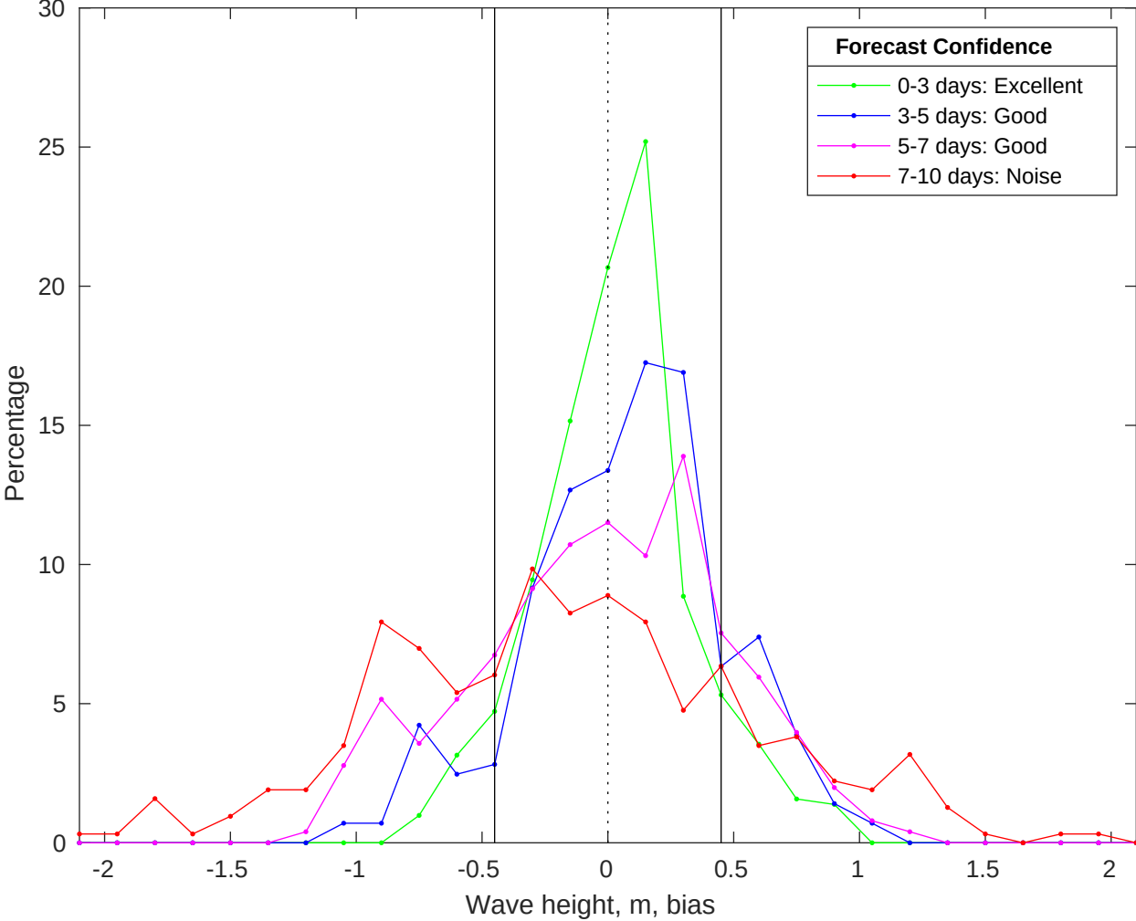
NDBC 46069 vs CMEMS Waves Bias Histogram: 10-Jan-2026
