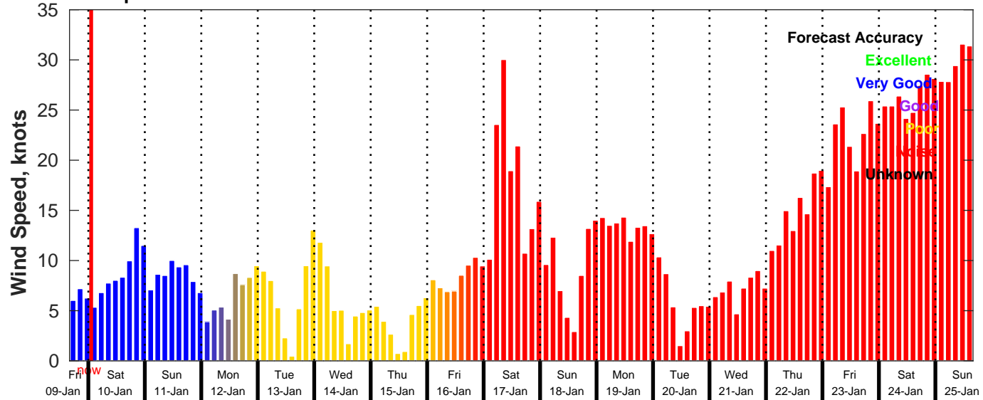
GFS Wind Speed Forecast for NDBC 46069 from 09-Jan-2026 16:00:00 to 25-Jan-2026 16:00:00
