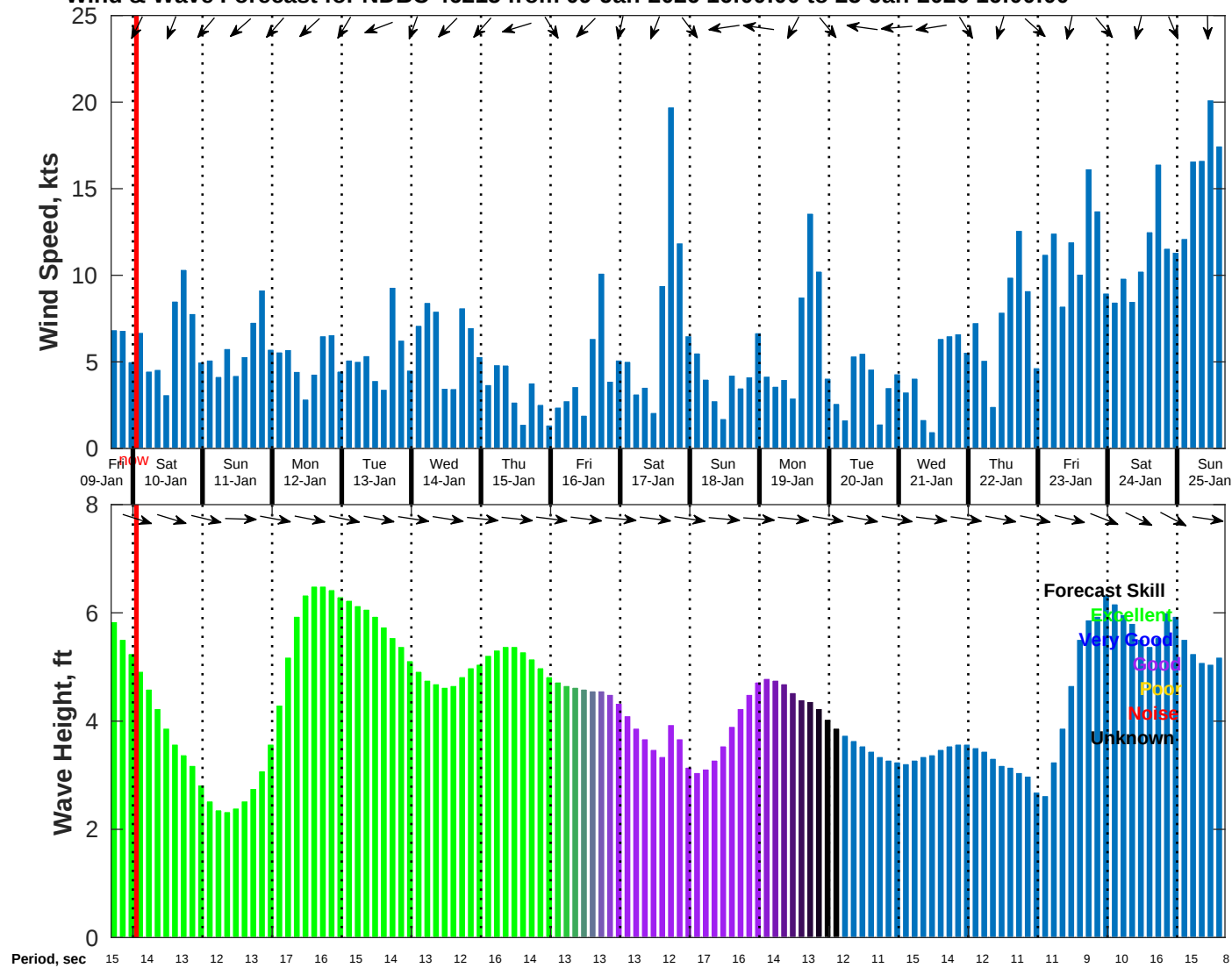
Wind & Wave Forecast for NDBC 46215 from 09-Jan-2026 16:00:00 to 25-Jan-2026 16:00:00
