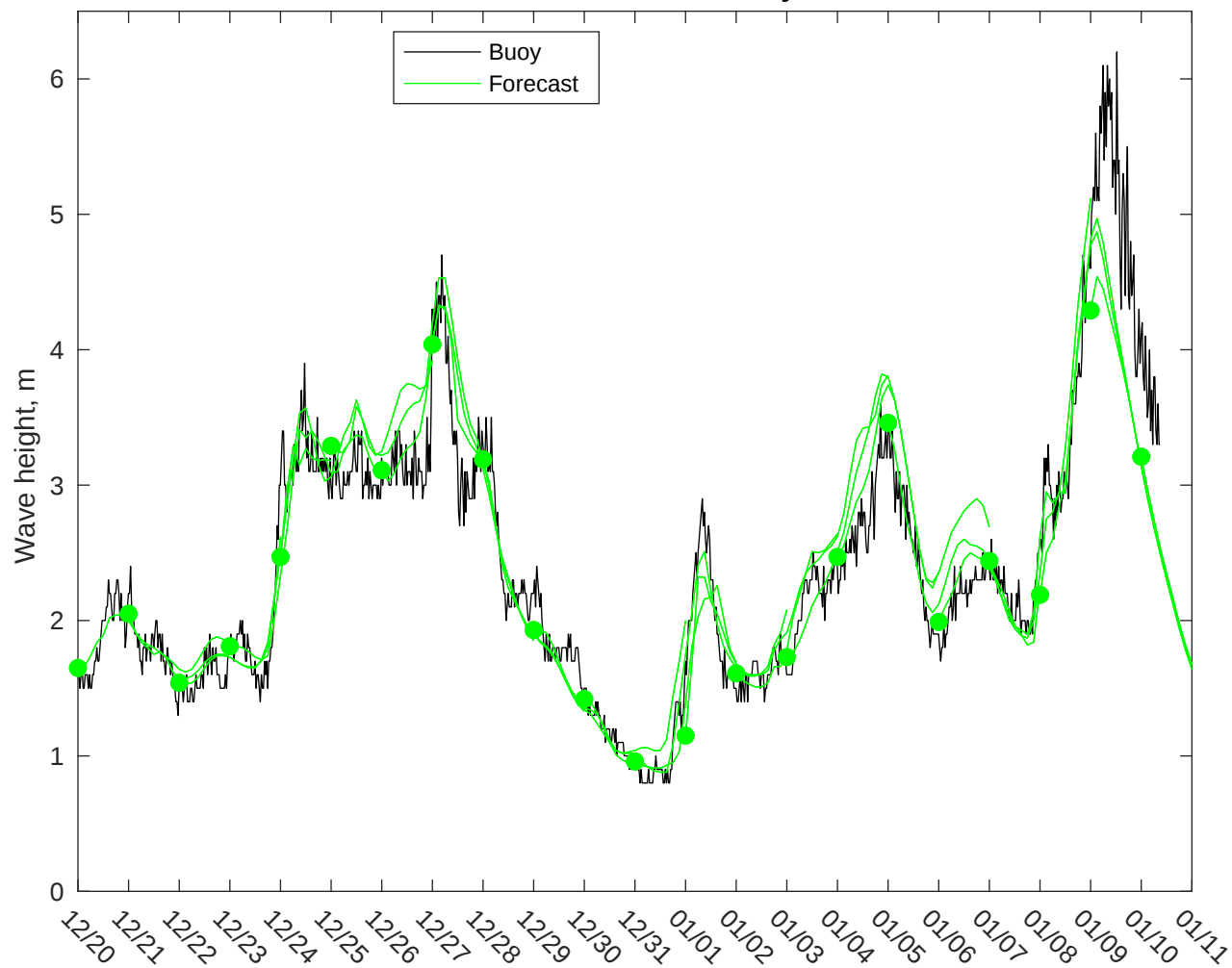
NDBC 46259 vs CMEMS Waves: 0 to 3 day forecast
