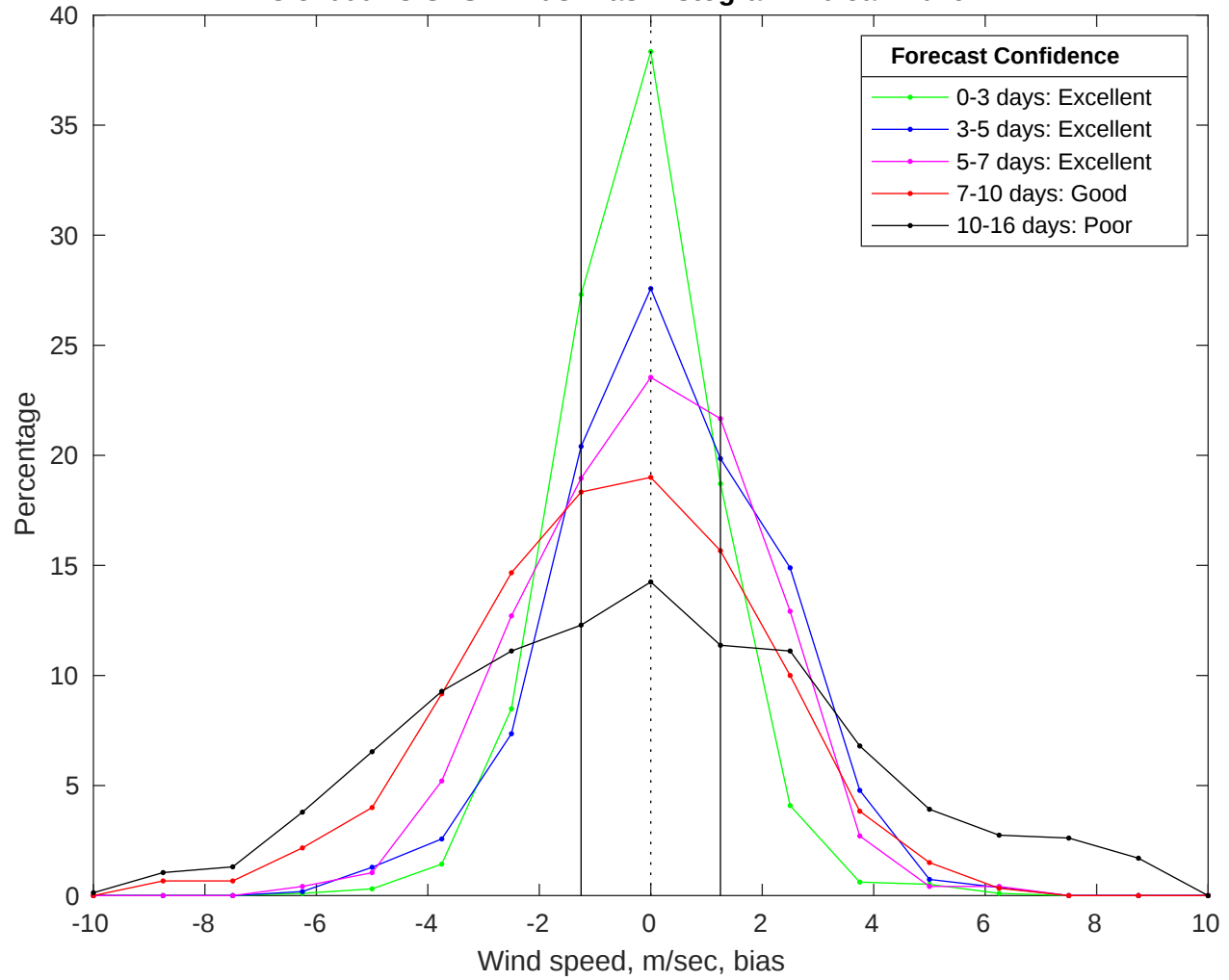
NDBC 51000 vs GFS Winds Bias Histogram: 10-Jan-2026
