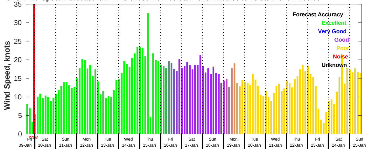
GFS Wind Speed Forecast for NDBC 51000 from 09-Jan-2026 14:00:00 to 25-Jan-2026 14:00:00
