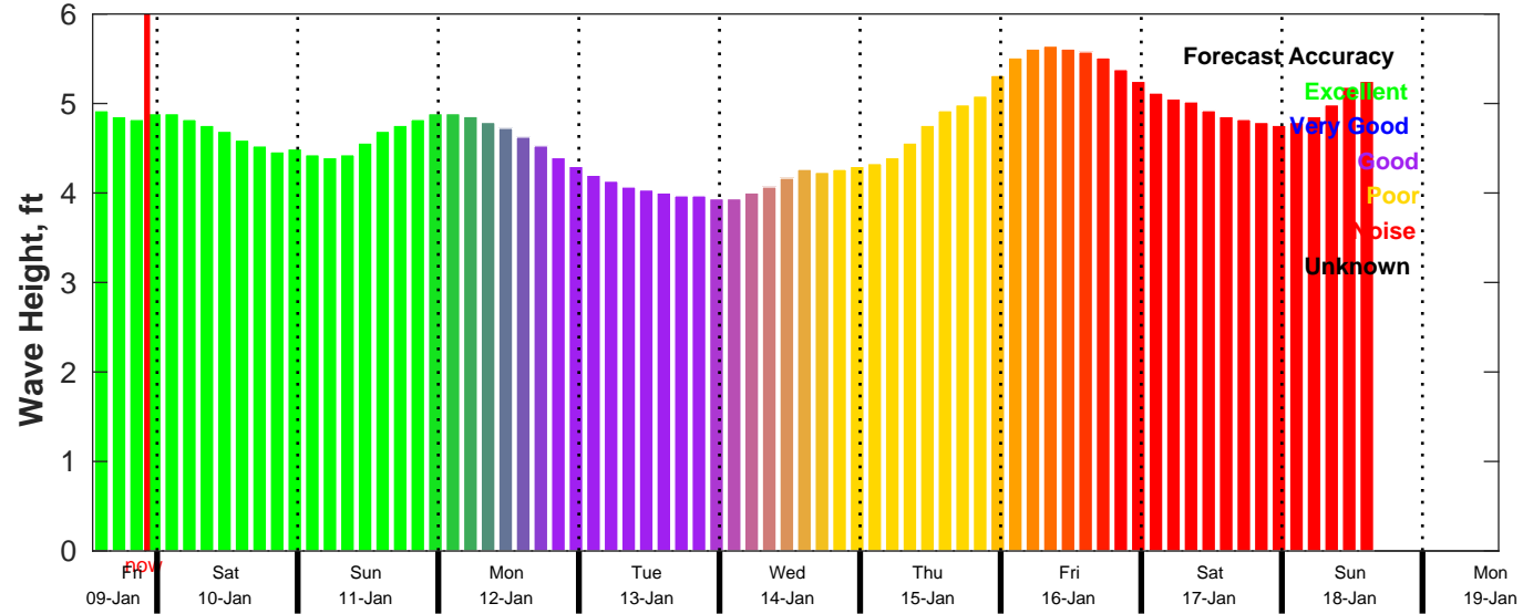
CMEMS Wave Forecast for NDBC 51209 from 09-Jan-2026 13:00:00 to 19-Jan-2026 13:00:00
