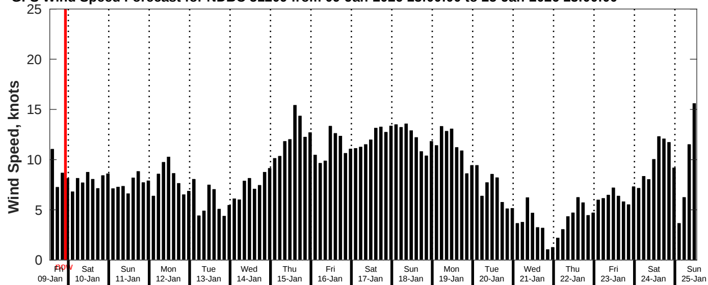
GFS Wind Speed Forecast for NDBC 51209 from 09-Jan-2026 13:00:00 to 25-Jan-2026 13:00:00
