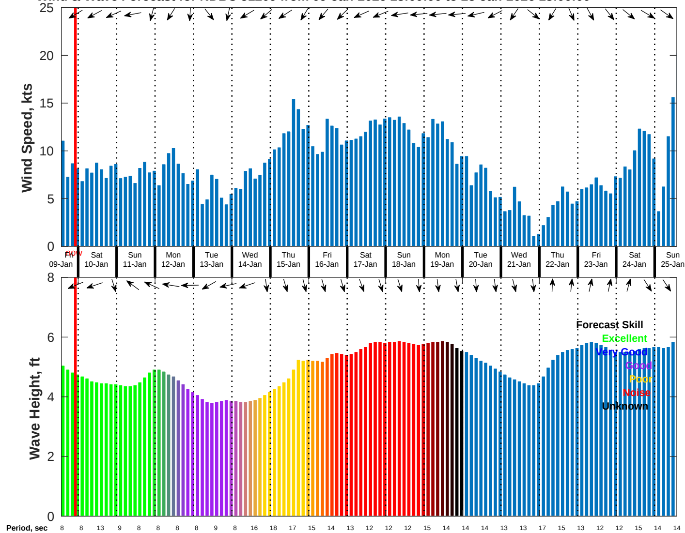
Wind & Wave Forecast for NDBC 51209 from 09-Jan-2026 13:00:00 to 25-Jan-2026 13:00:00
