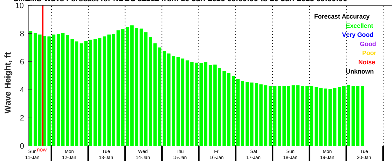
CMEMS Wave Forecast for NDBC 52212 from 10-Jan-2026 09:00:00 to 20-Jan-2026 09:00:00
