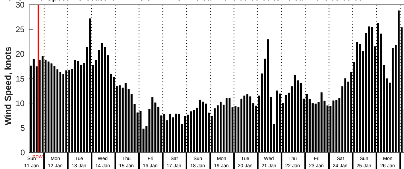
GFS Wind Speed Forecast for NDBC 52212 from 10-Jan-2026 09:00:00 to 26-Jan-2026 09:00:00
