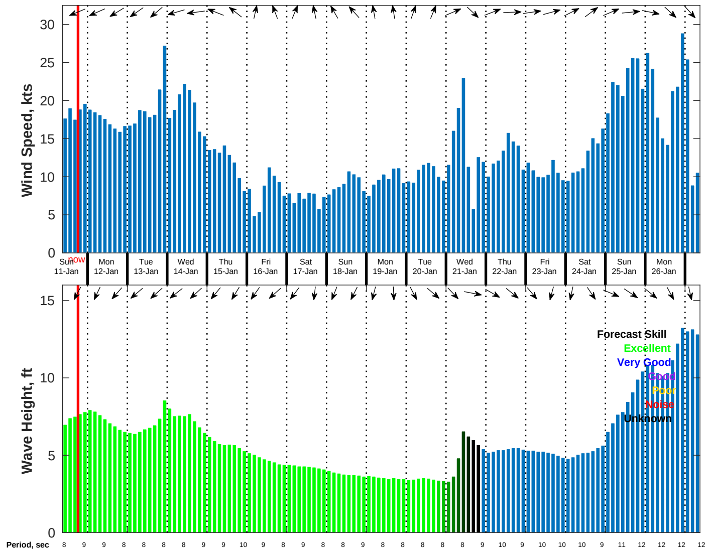
Wind & Wave Forecast for NDBC 52212 from 10-Jan-2026 09:00:00 to 26-Jan-2026 09:00:00
