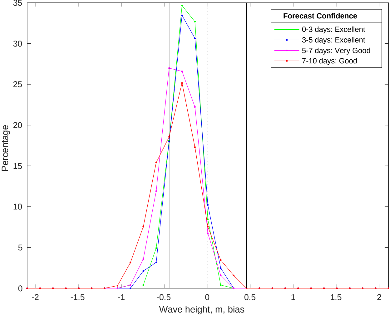
NDBC 52213 vs CMEMS Waves Bias Histogram: 10-Jan-2026
