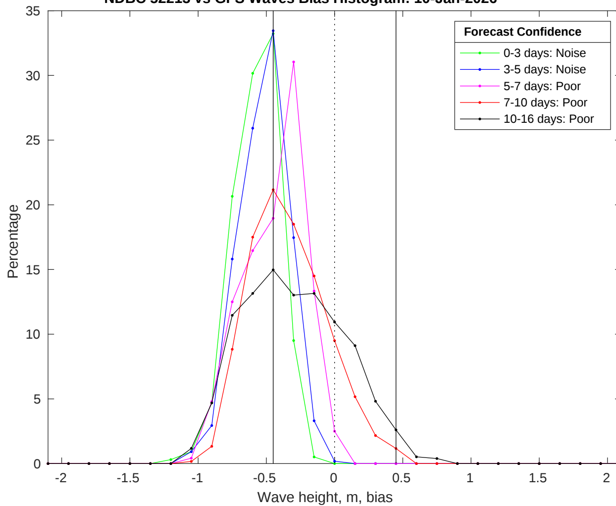
NDBC 52213 vs GFS Waves Bias Histogram: 10-Jan-2026
