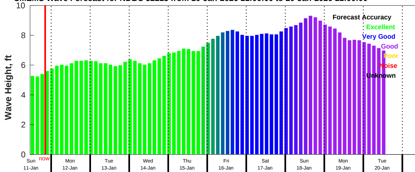
CMEMS Wave Forecast for NDBC 52213 from 10-Jan-2026 11:00:00 to 20-Jan-2026 11:00:00
