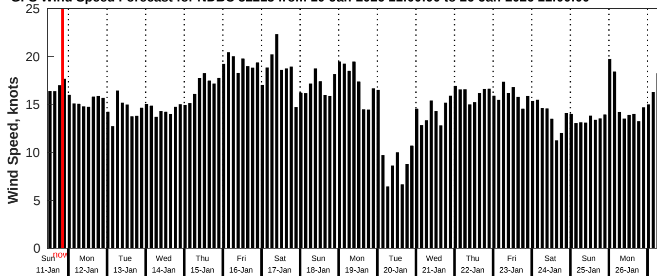
GFS Wind Speed Forecast for NDBC 52213 from 10-Jan-2026 11:00:00 to 26-Jan-2026 11:00:00
