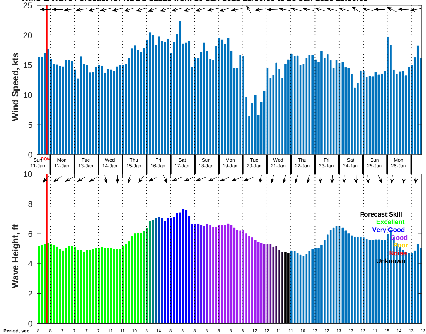
Wind & Wave Forecast for NDBC 52213 from 10-Jan-2026 11:00:00 to 26-Jan-2026 11:00:00
