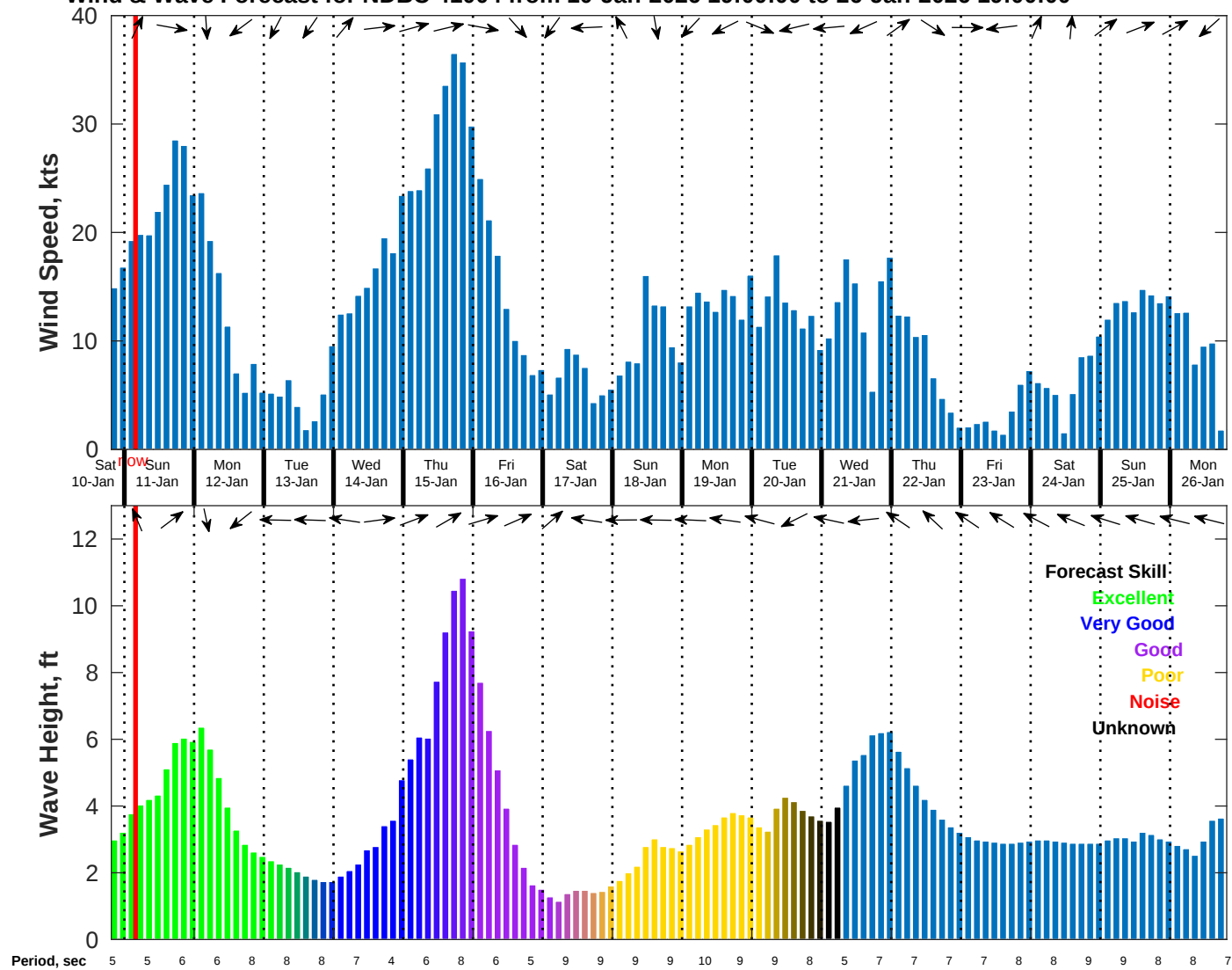
Wind & Wave Forecast for NDBC 41004 from 10-Jan-2026 19:00:00 to 26-Jan-2026 19:00:00
