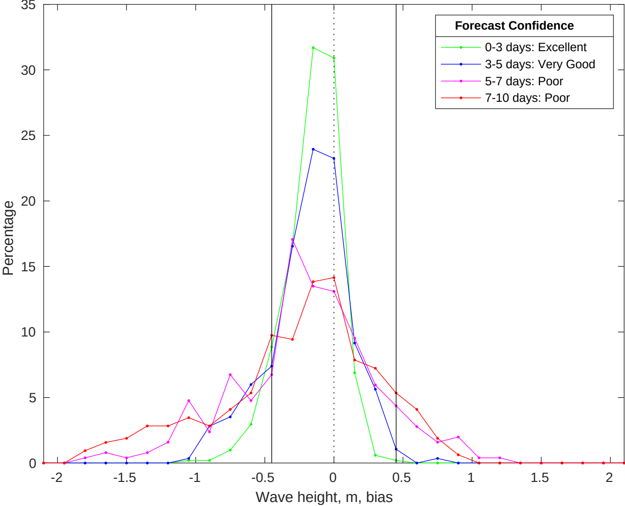
NDBC 41013 vs CMEMS Waves Bias Histogram: 11-Jan-2026
