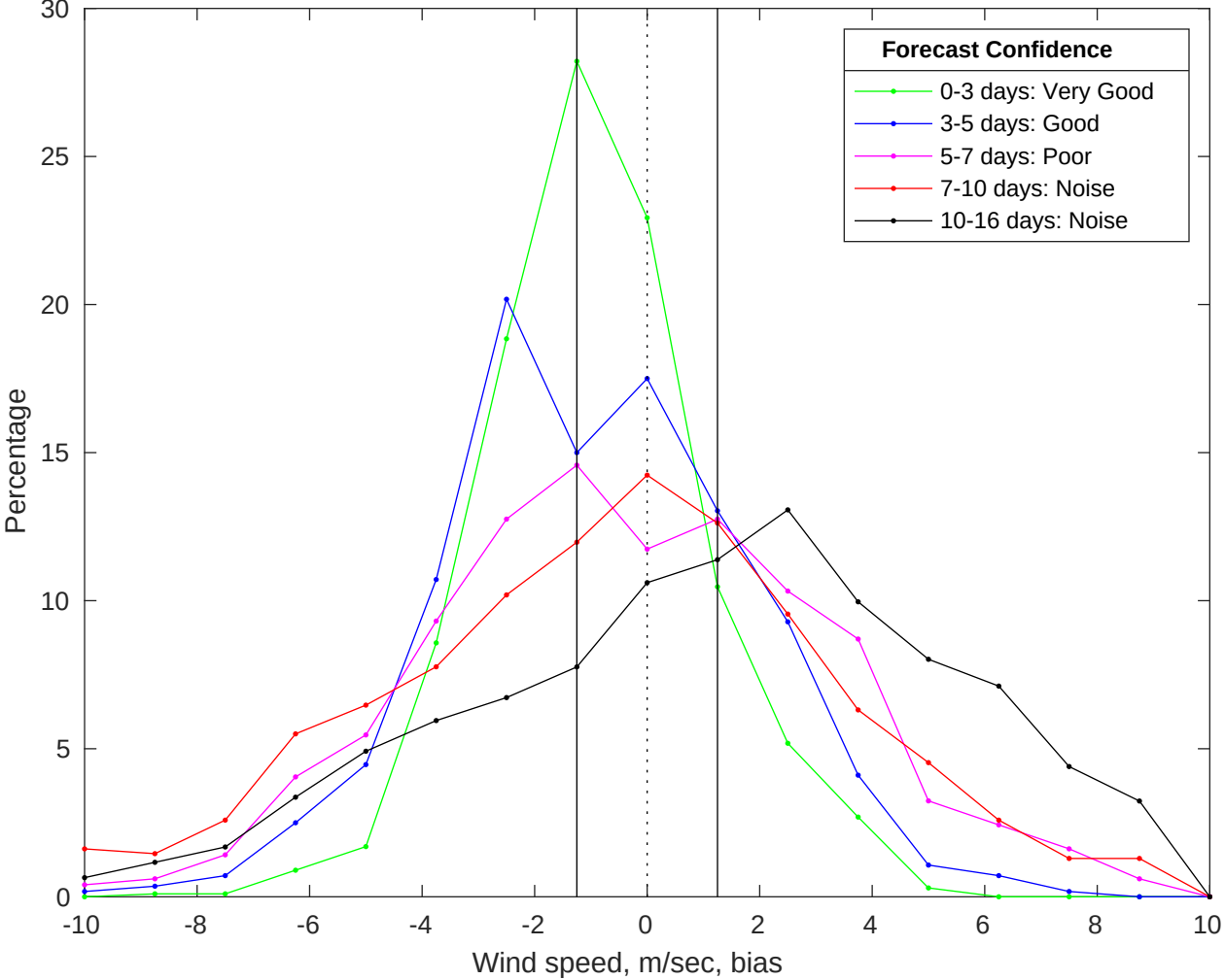
NDBC 41013 vs GFS Winds Bias Histogram: 11-Jan-2026
