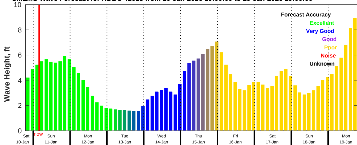
CMEMS Wave Forecast for NDBC 41013 from 10-Jan-2026 19:00:00 to 19-Jan-2026 19:00:00
