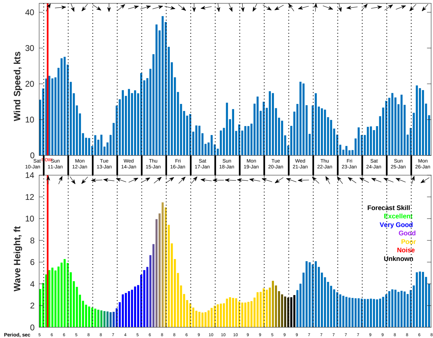
Wind & Wave Forecast for NDBC 41013 from 10-Jan-2026 19:00:00 to 26-Jan-2026 19:00:00
