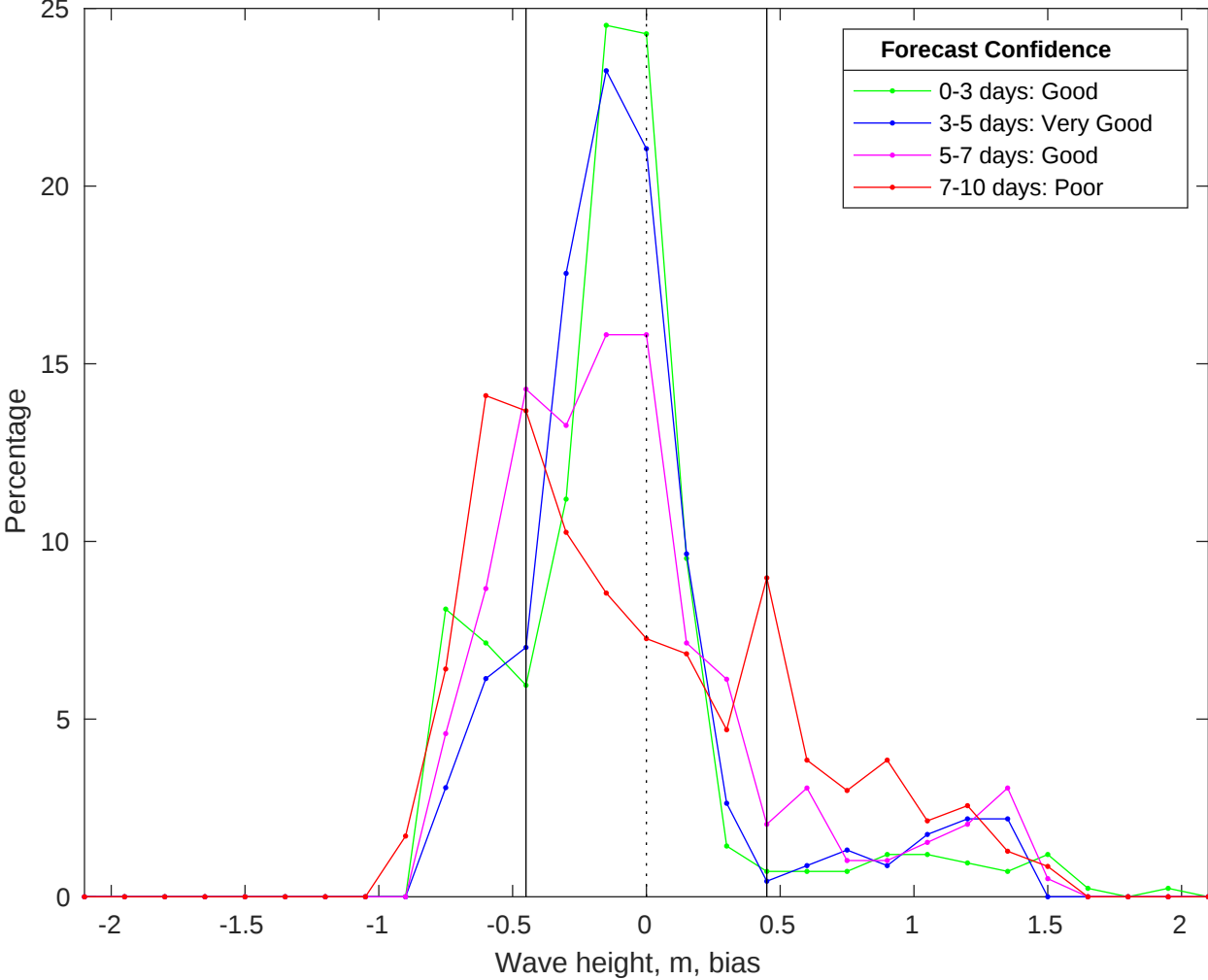
NDBC 42020 vs CMEMS Waves Bias Histogram: 07-Jan-2026
