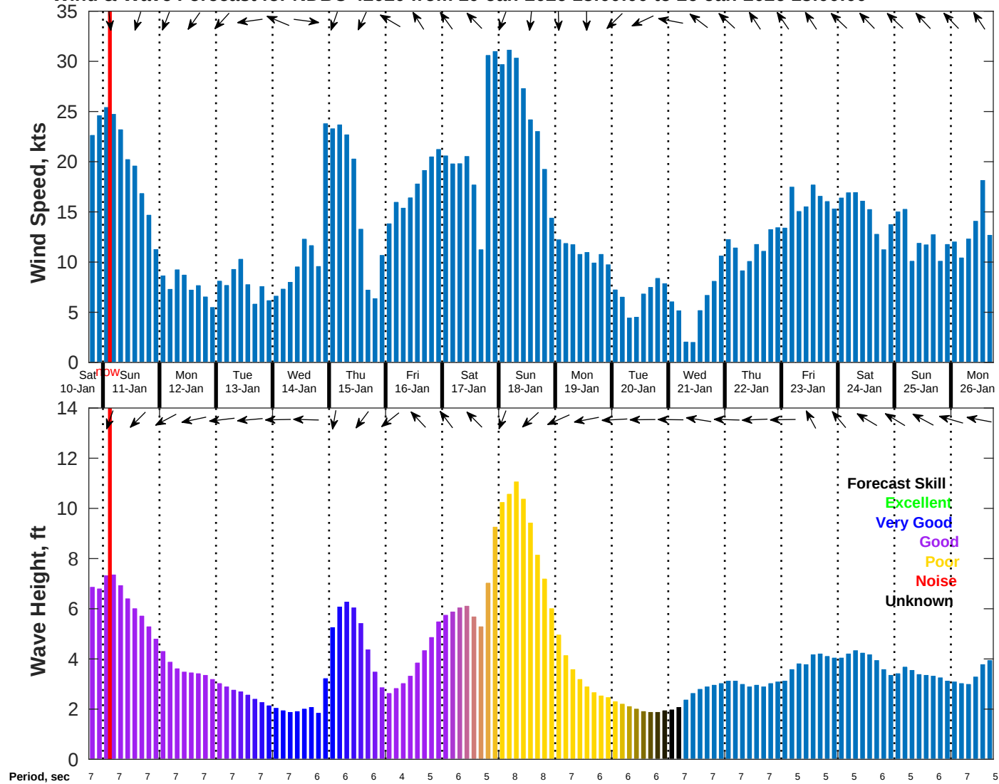
Wind & Wave Forecast for NDBC 42020 from 10-Jan-2026 18:00:00 to 26-Jan-2026 18:00:00
