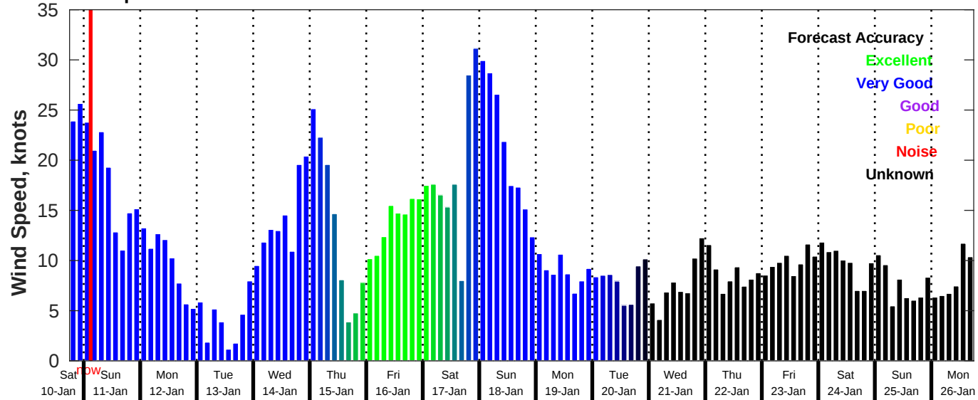
GFS Wind Speed Forecast for NDBC 42035 from 10-Jan-2026 18:00:00 to 26-Jan-2026 18:00:00
