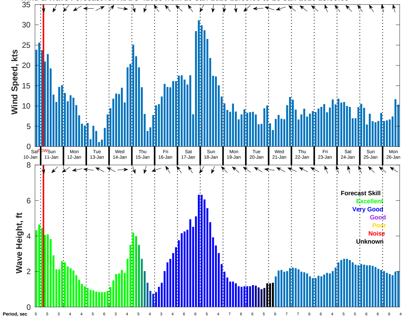
Wind & Wave Forecast for NDBC 42035 from 10-Jan-2026 18:00:00 to 26-Jan-2026 18:00:00
