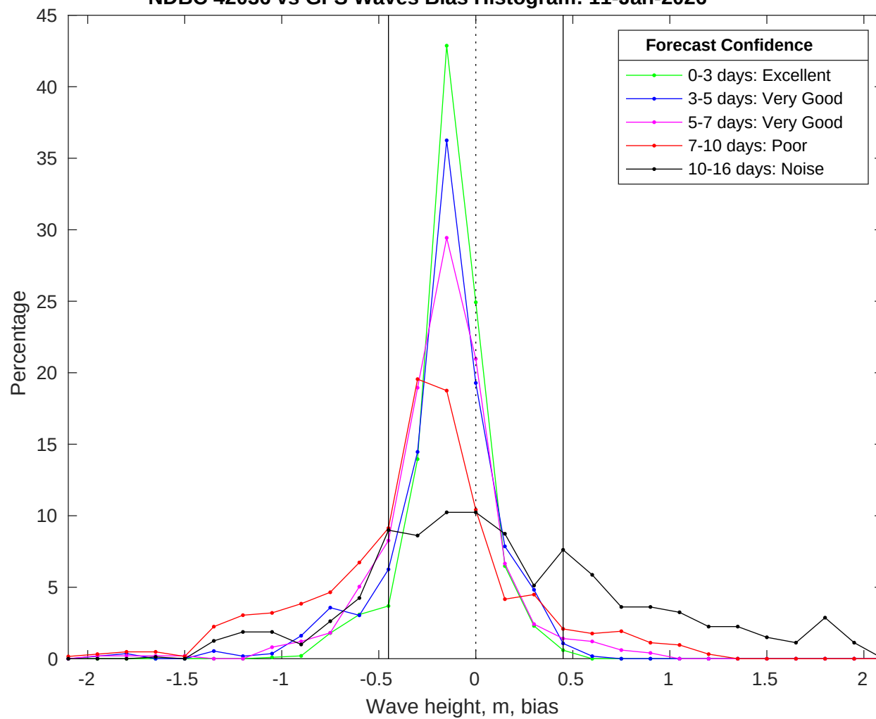
NDBC 42036 vs GFS Waves Bias Histogram: 11-Jan-2026
