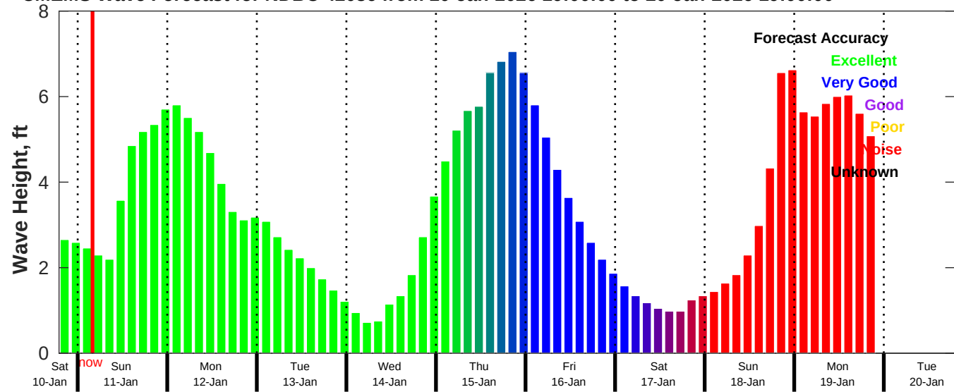
CMEMS Wave Forecast for NDBC 42036 from 10-Jan-2026 19:00:00 to 20-Jan-2026 19:00:00
