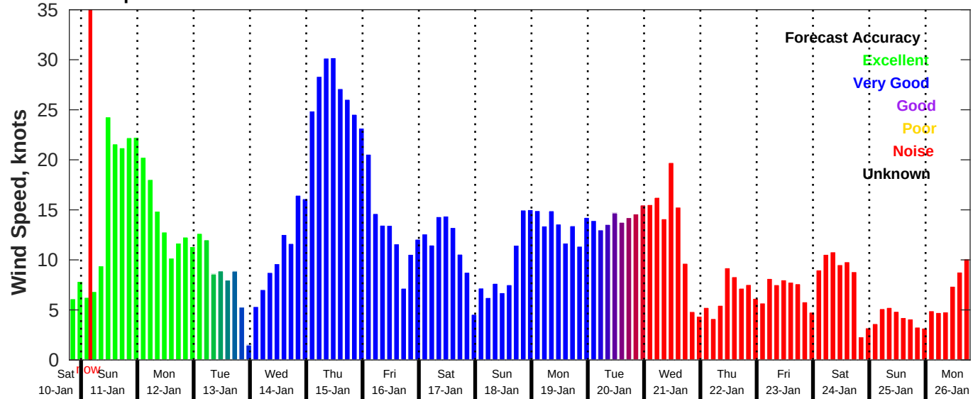
GFS Wind Speed Forecast for NDBC 42036 from 10-Jan-2026 19:00:00 to 26-Jan-2026 19:00:00
