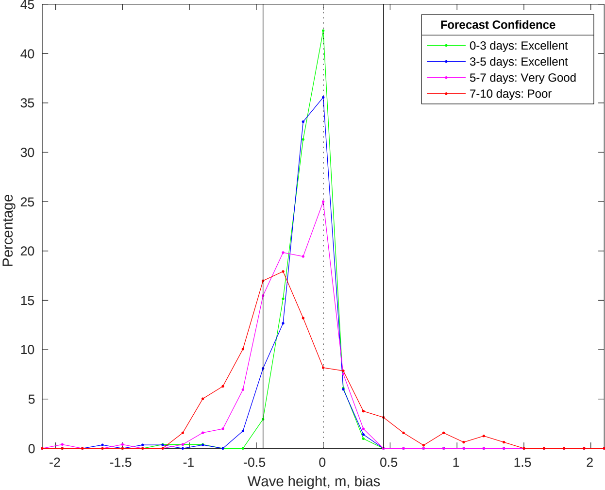
NDBC 42040 vs CMEMS Waves Bias Histogram: 11-Jan-2026
