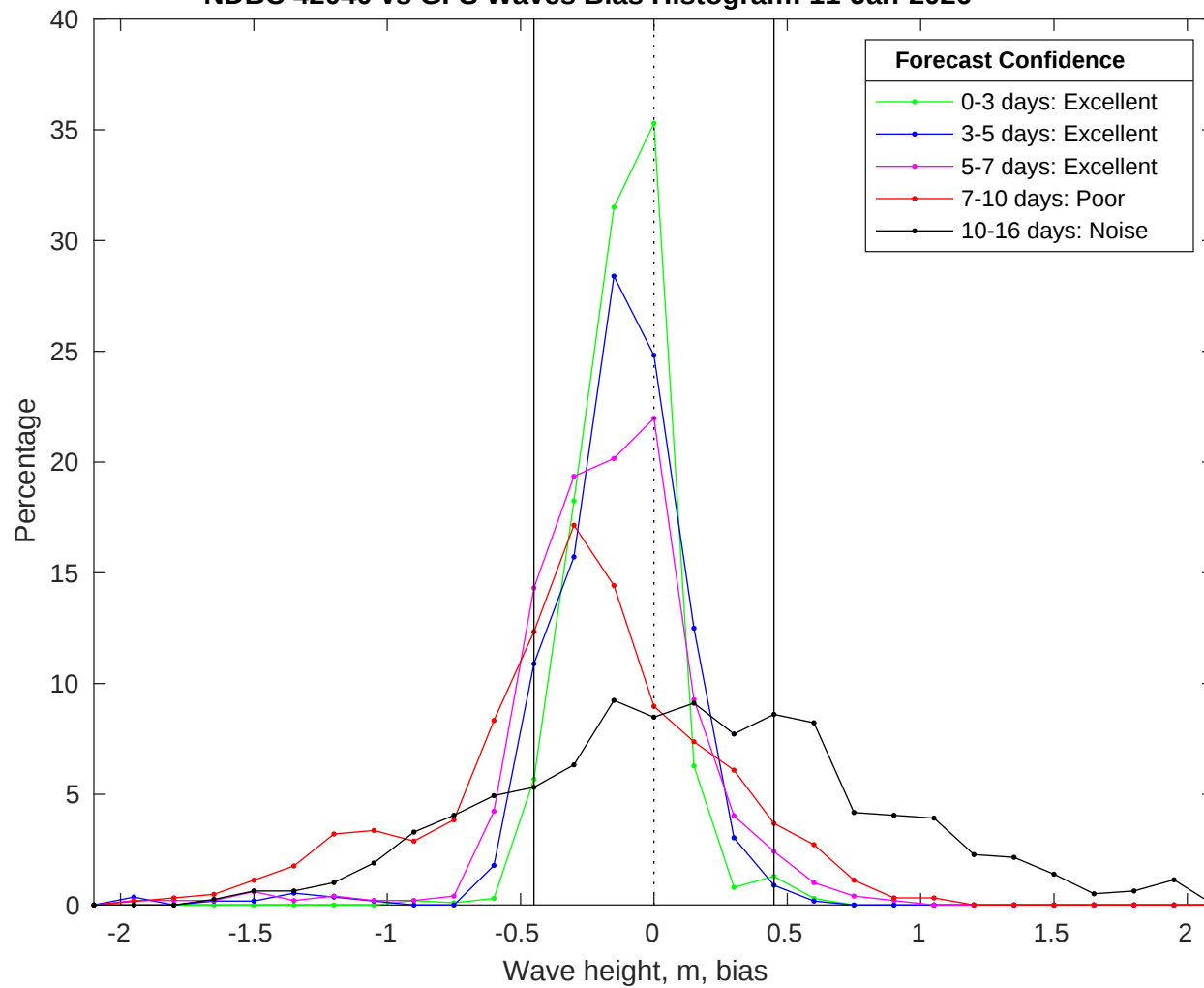
NDBC 42040 vs GFS Waves Bias Histogram: 11-Jan-2026
