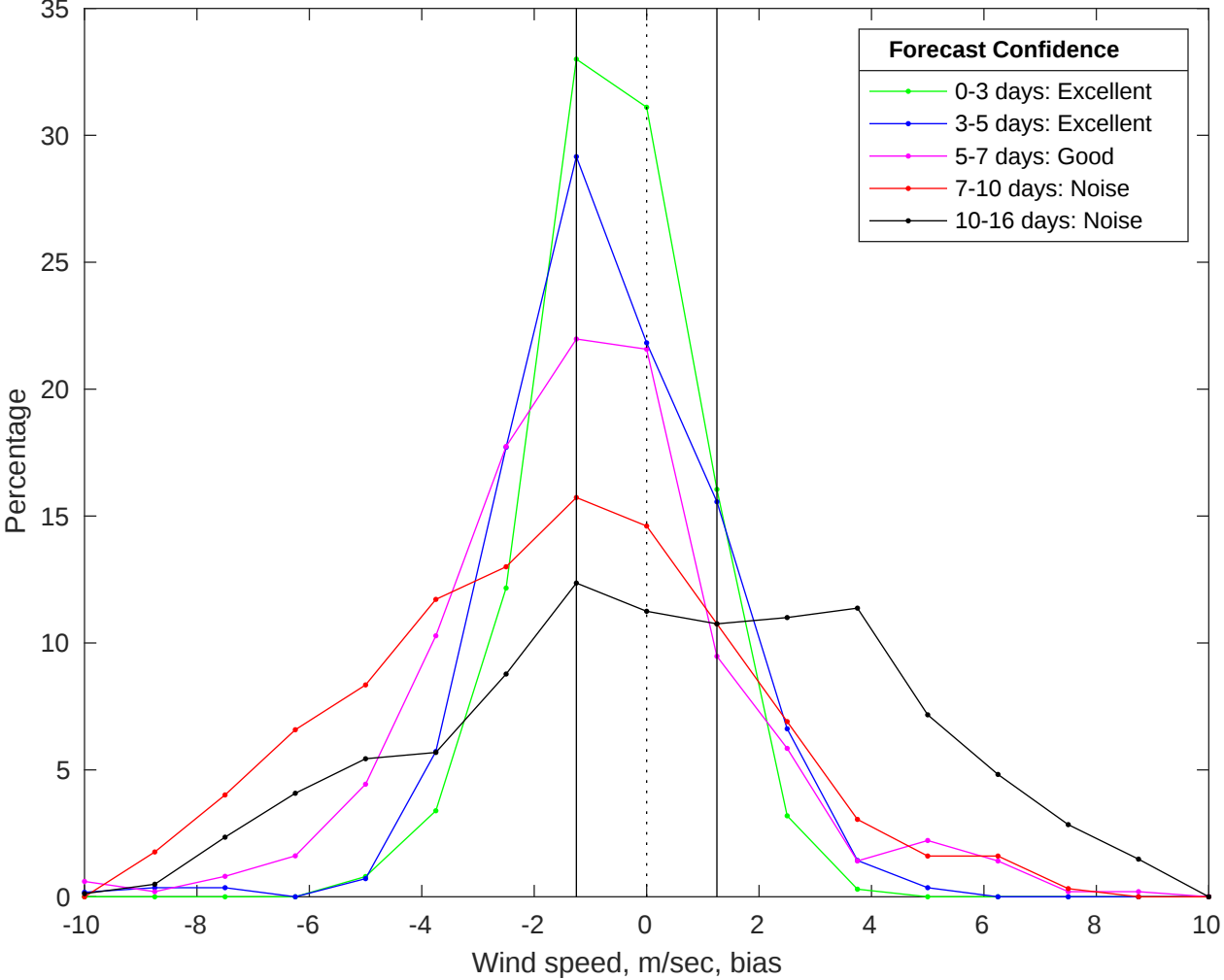
NDBC 42040 vs GFS Winds Bias Histogram: 11-Jan-2026
