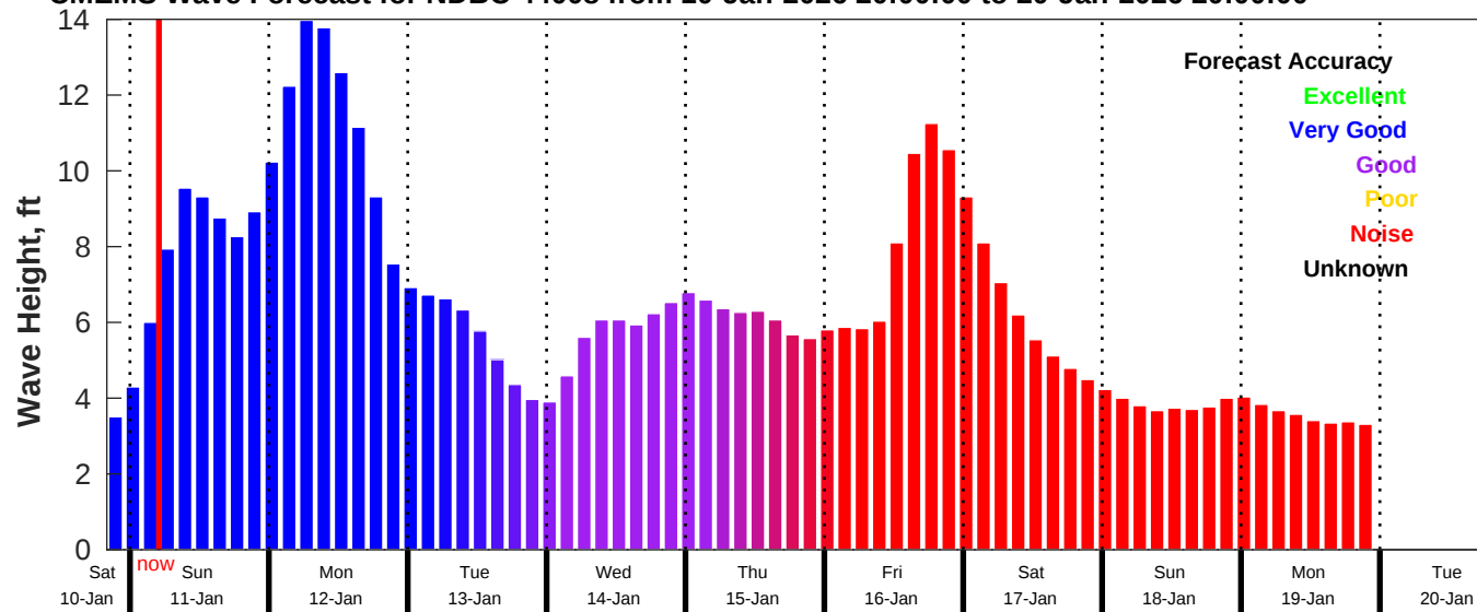
CMEMS Wave Forecast for NDBC 44008 from 10-Jan-2026 20:00:00 to 20-Jan-2026 20:00:00
