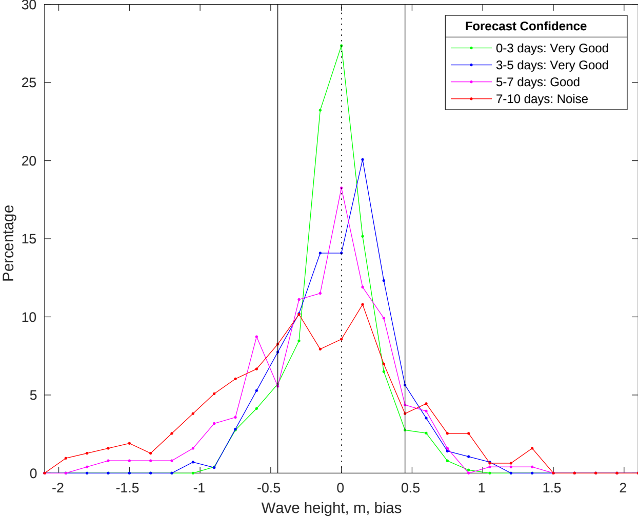
NDBC 46011 vs CMEMS Waves Bias Histogram: 11-Jan-2026
