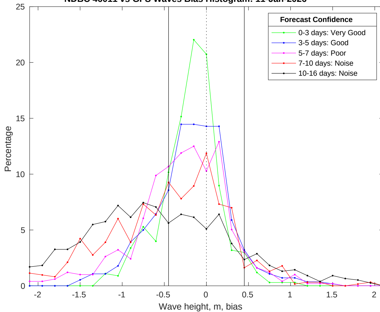
NDBC 46011 vs GFS Waves Bias Histogram: 11-Jan-2026
