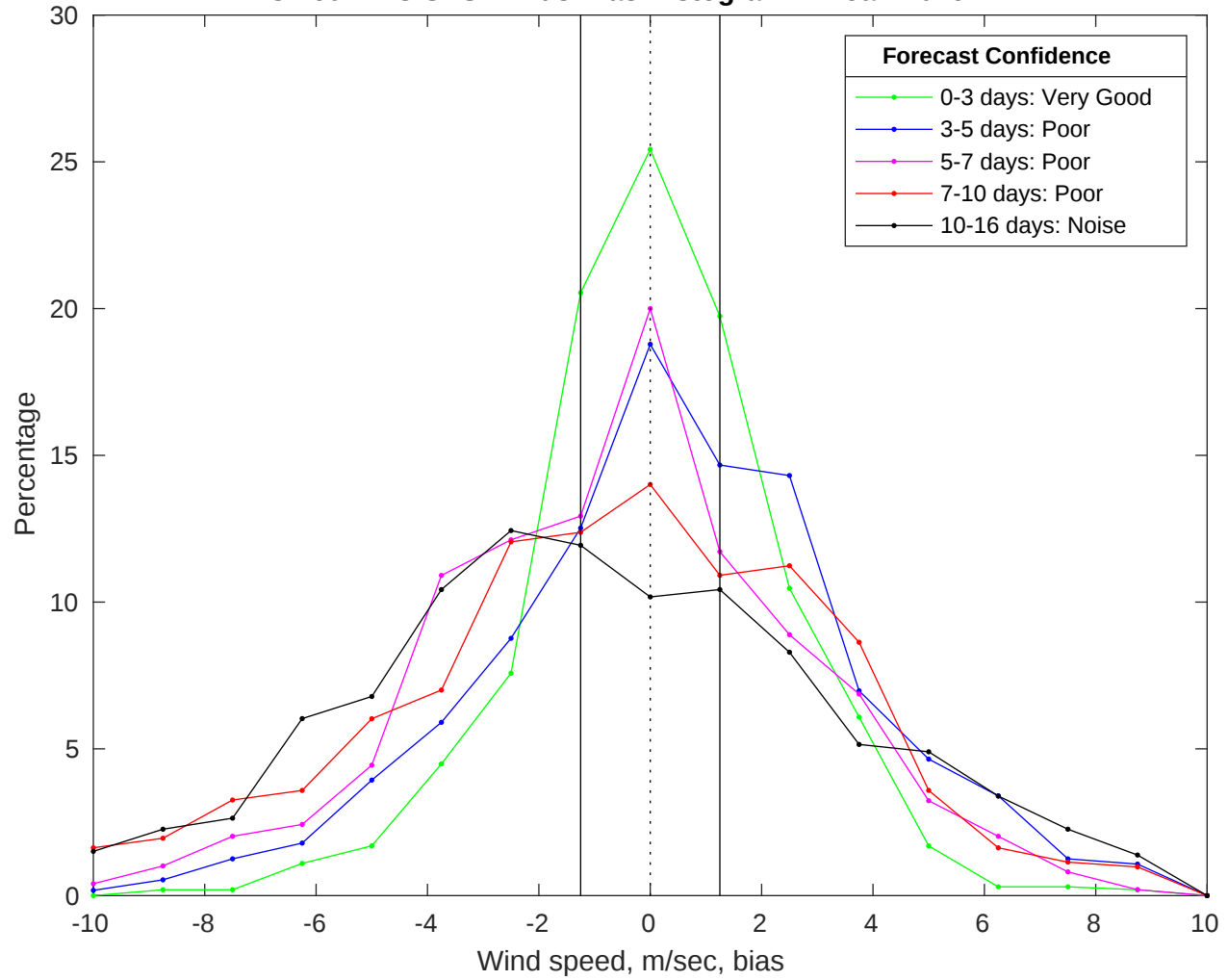
NDBC 46011 vs GFS Winds Bias Histogram: 11-Jan-2026
