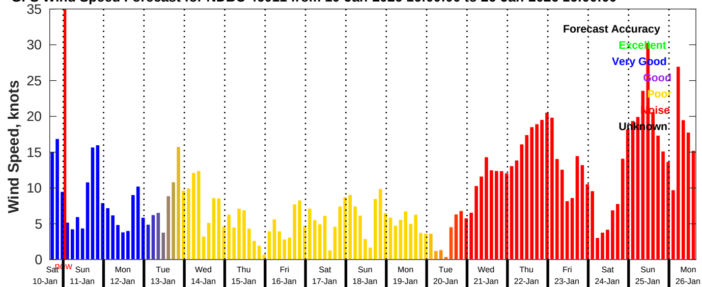
GFS Wind Speed Forecast for NDBC 46011 from 10-Jan-2026 16:00:00 to 26-Jan-2026 16:00:00
