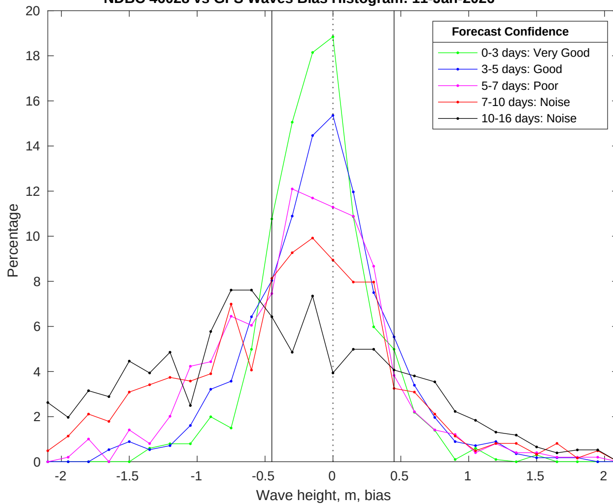
NDBC 46028 vs GFS Waves Bias Histogram: 11-Jan-2026
