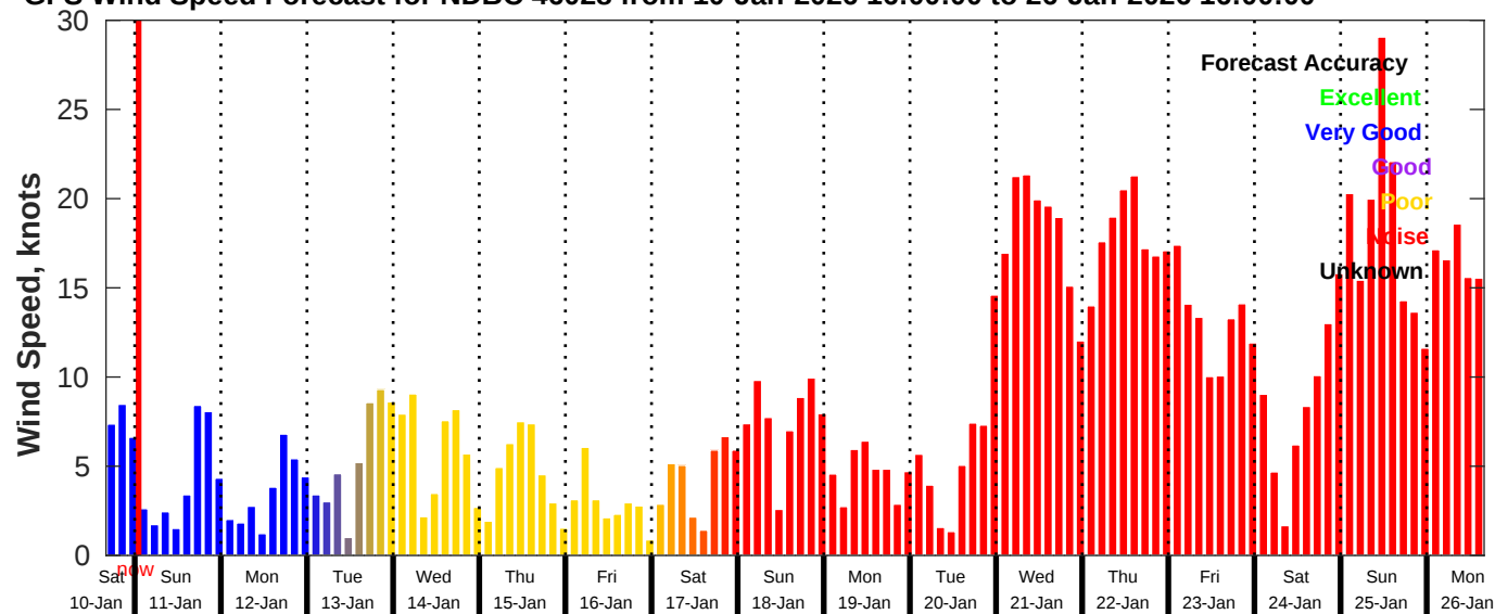
GFS Wind Speed Forecast for NDBC 46028 from 10-Jan-2026 16:00:00 to 26-Jan-2026 16:00:00
