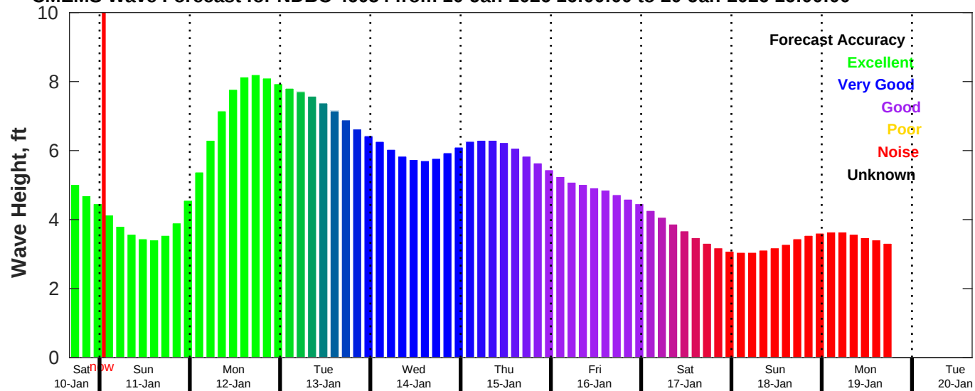
CMEMS Wave Forecast for NDBC 46054 from 10-Jan-2026 16:00:00 to 20-Jan-2026 16:00:00
