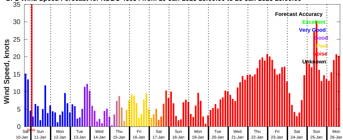
GFS Wind Speed Forecast for NDBC 46054 from 10-Jan-2026 16:00:00 to 26-Jan-2026 16:00:00
