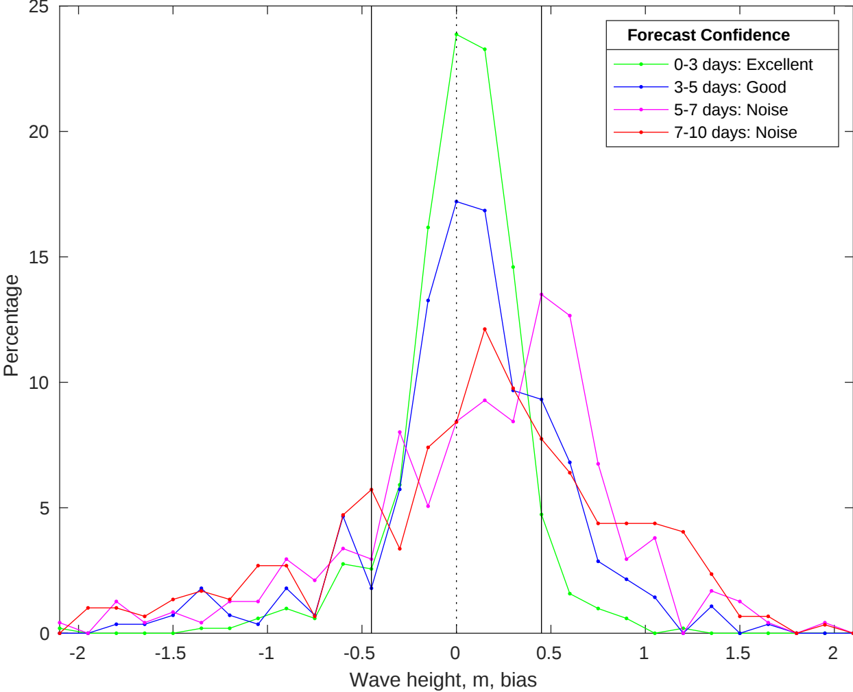
NDBC 46059 vs CMEMS Waves Bias Histogram: 11-Jan-2026
