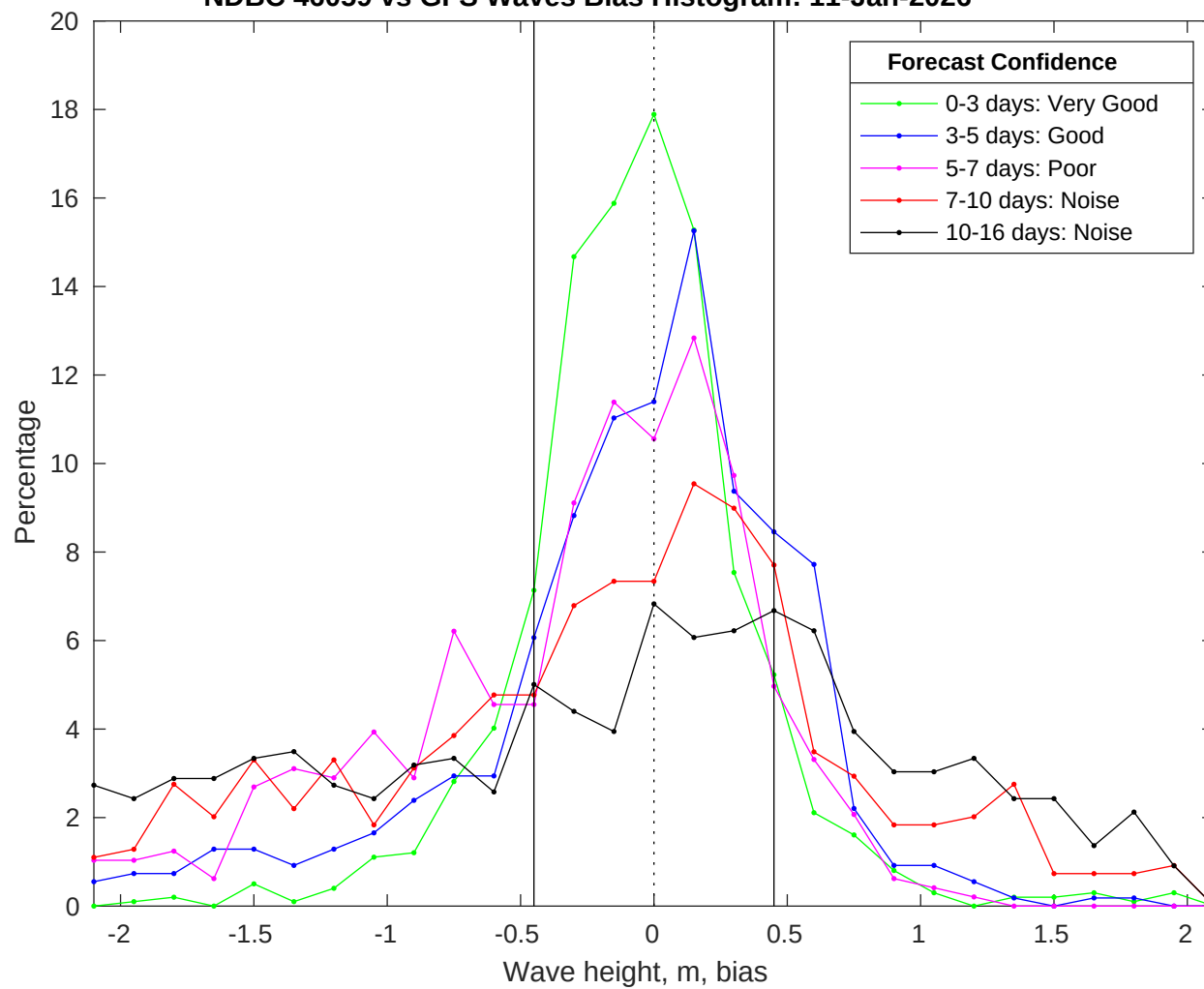
NDBC 46059 vs GFS Waves Bias Histogram: 11-Jan-2026
