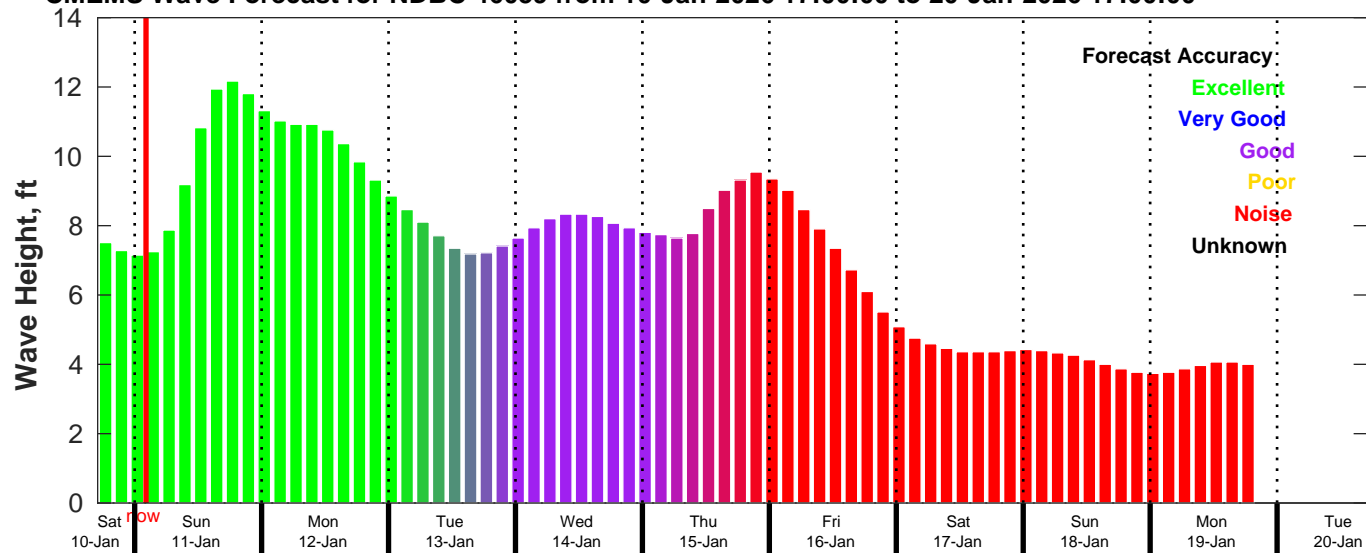
CMEMS Wave Forecast for NDBC 46059 from 10-Jan-2026 17:00:00 to 20-Jan-2026 17:00:00
