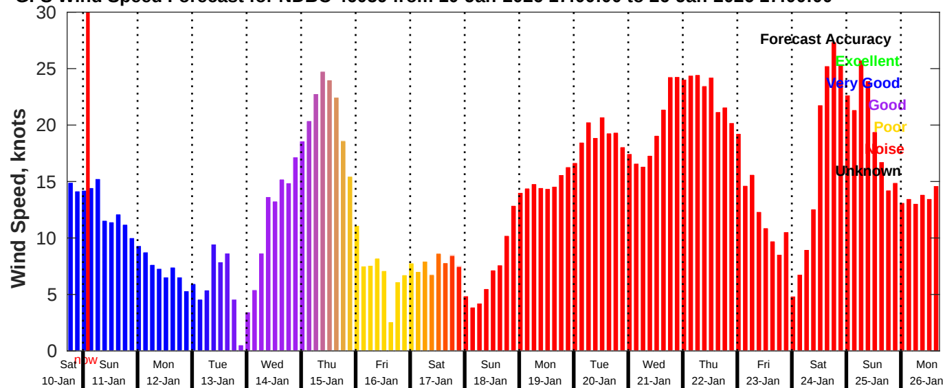
GFS Wind Speed Forecast for NDBC 46059 from 10-Jan-2026 17:00:00 to 26-Jan-2026 17:00:00
