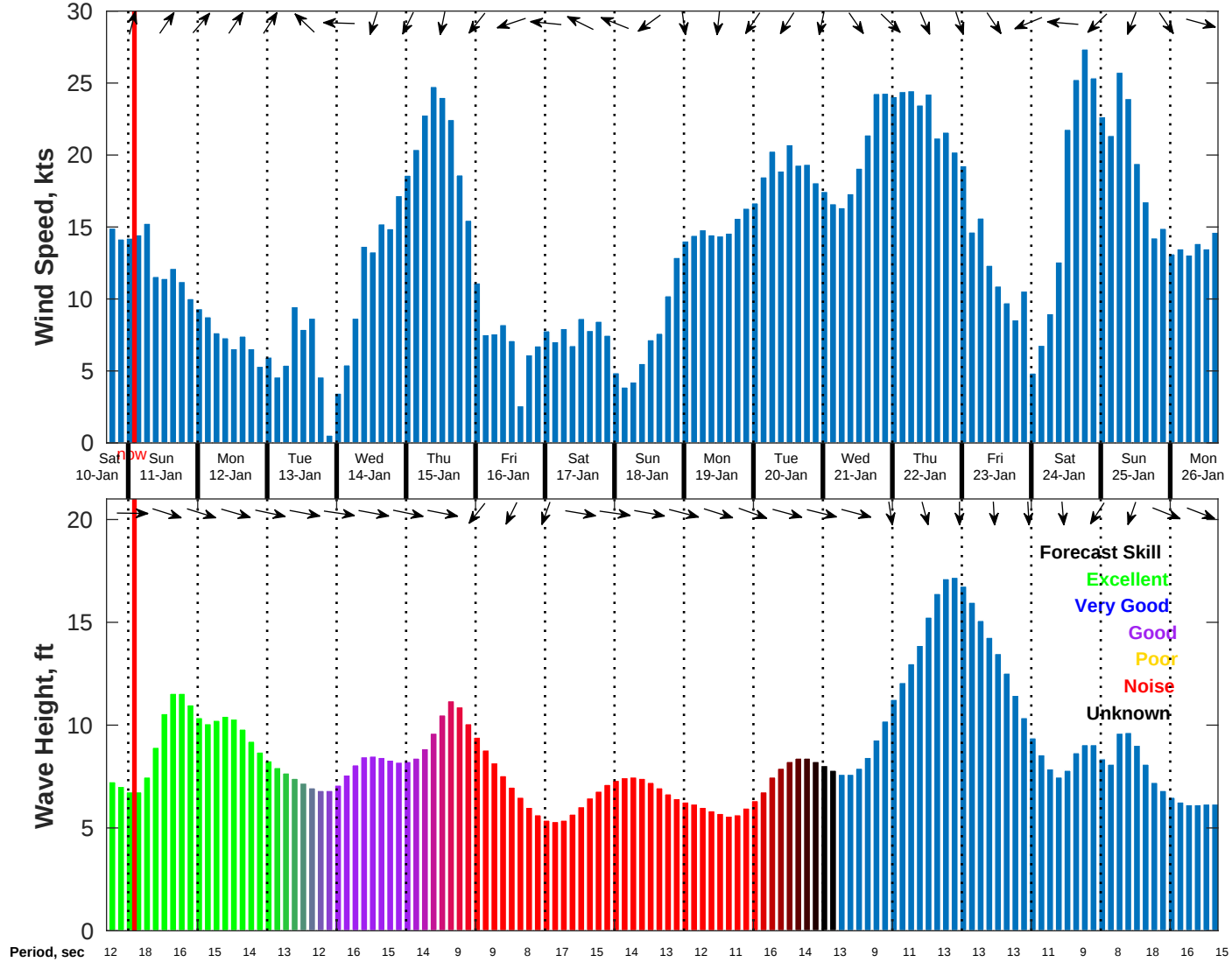
Wind & Wave Forecast for NDBC 46059 from 10-Jan-2026 17:00:00 to 26-Jan-2026 17:00:00
